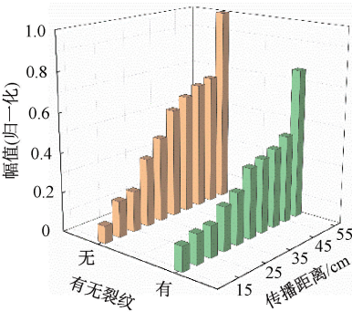
(b) 1.0 MHz 频率下有无裂纹能量衰减模型 (b) Crack energy attenuation model at 1.0 MHz frequency
